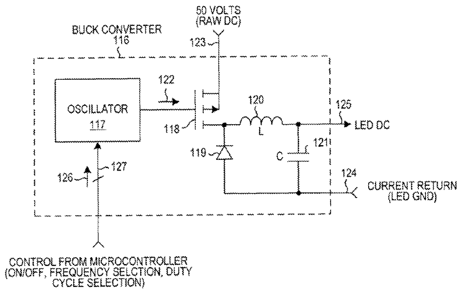
BUCK CONVERTER
